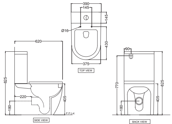
OPS-WHT-15753P180UFSMZ Rimless Bowl with Cistern for Coupled WC with UF Soft Close Slim Seat Cover, Hinges, Dual Flush Cistern Fitting and Fixing Accessories, Size: 390x620x825 mm, P Trap- 180 mm
