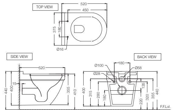
SLS-WHT-6953BIPPSM Rimless, Blind Installation Wall Hung WC with PP Soft Close Slim Seat Cover, Hinges and Accessories Set, Size: 375x520x400 mm
