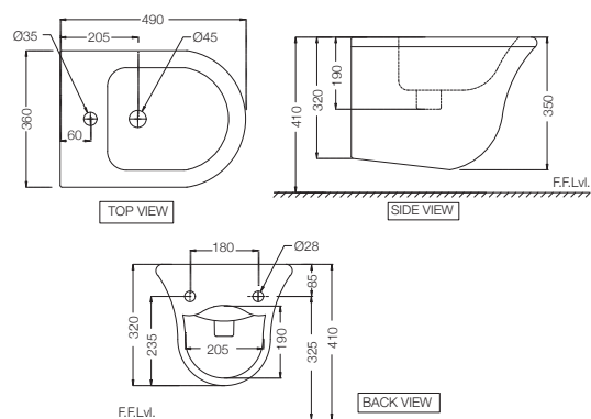
ONS-WHT-10153 Blind Installation Wall Hung Bidet with Accessories Set, Size: 360x490x350 mm
