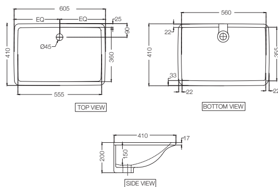
FNS-WHT-40701 Under Counter Basin with Fixing Accessories, Size: 605x410x200 mm, Shape: Rectangular
