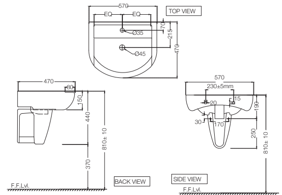
ARS-WHT-39801 Wall Hung Basin with Fixing Accessories, Size: 570x470x190 mm ARS-WHT-39305 Half Pedestal with Fixing Accessories for ARS-WHT-39801
