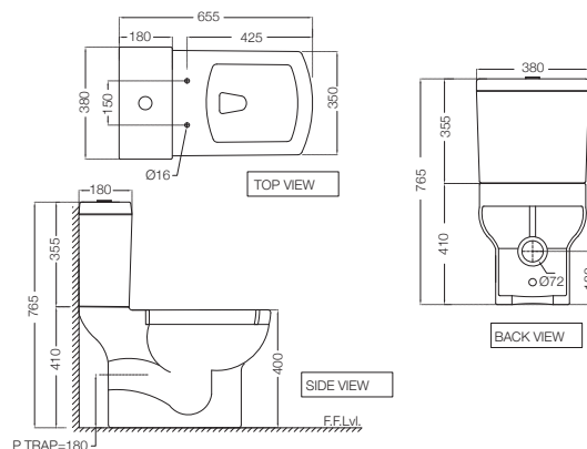
LYS-WHT-38751P180UFSMZ Bowl with Cistern for Coupled WC with UF Soft Close Slim Seat Cover, Hinges, Dual Flush Cistern Fitting and Fixing Accessories, Size: 380x655x765 mm, P Trap- 180 mm
