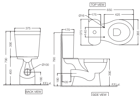
SLS-WHT-6751P180PPZ Bowl with Cistern for Coupled WC with PP Soft Close Seat Cover, Hinges, Dual Flush Cistern Fitting, Fixing Accessories and Accessories Set, Size: 375x650x790 mm, P Trap- 180 mm
