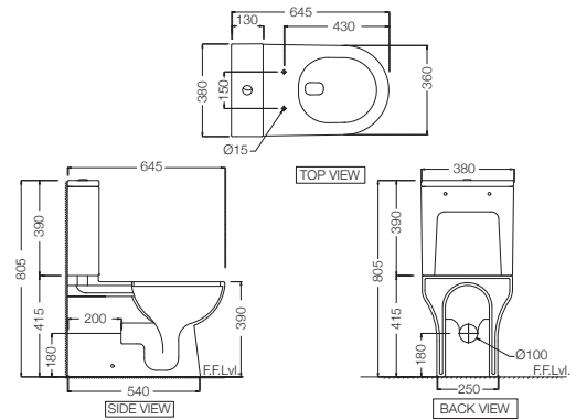
OPS-WHT-15753NP180UFSMZ Rimless Bowl with Cistern for Coupled WC with UF Soft Close Slim Seat Cover, Hinges, Dual Flush Cistern Fitting and Fixing Accessories Set, Size: 380x645x805 mm, P Trap- 180 mm
