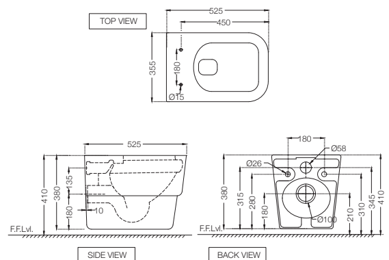
DRS-WHT-37953BIUFMS Rimless, Blind Installation Wall Hung WC with UF Soft Close Slim Seat Cover, Hinges and Accessories Set, Size: 355x525x380 mm
