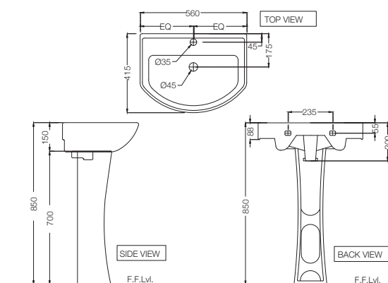
CNS-WHT-801 Wall Hung Basin with Fixing Accessories, Size: 560x415x200 mm CNS-WHT-301 Full Pedestal for CNS-WHT-801
