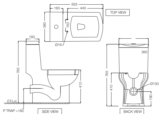
LYS-WHT-38851P180UFSM Single Piece WC with UF Soft Close Slim Seat Cover, Hinges, Dual Flush Cistern Fitting, Fixing Accessories, Size: 360x655x765 mm, P Trap- 180 mm
