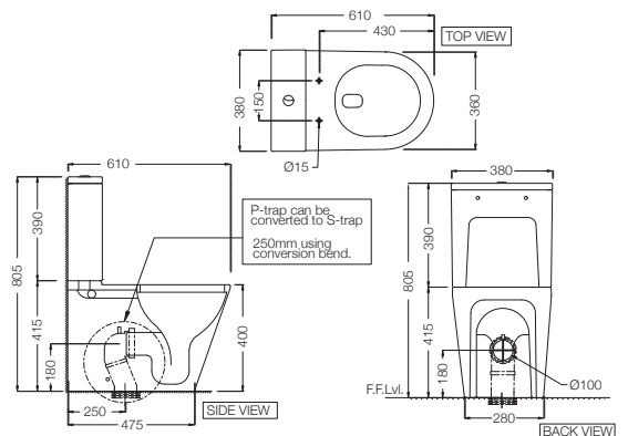
VGS-WHT-81753S250UFSMZ Rimless Bowl with Cistern for Coupled WC with UF Soft Close Slim Seat Cover, Hinges, Dual Flush Cistern Fitting, Conversion Bend, Fixing Accessories and Accessories Set, Size: 380x610x805 mm, S Trap- 250 mm (with Conversion Bend)
