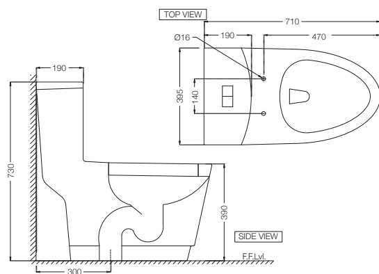
VGS-WHT-81853S300UF Rimless Single Piece WC with UF Soft Close Seat Cover, Hinges, Dual Flush Cistern Fitting, Fixing Accessories and Accessories Set, Size: 395x710x730 mm, S Trap- 300 mm
