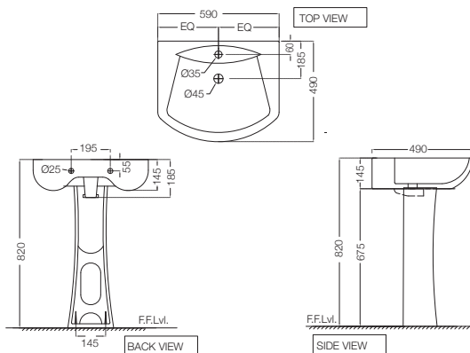
LYS-WHT-38801 Wall Hung Basin with Fixing Accessories, Size: 590x490x185 mm LYS-WHT-38301 Full Pedestal for LYS-WHT-38801
