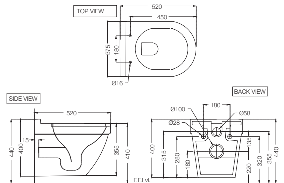
SLS-WHT-6953BIUFMS Rimless, Blind Installation Wall Hung WC with UF Soft Close Slim Seat Cover, Hinges and Accessories Set, Size: 375x520x400 mm
