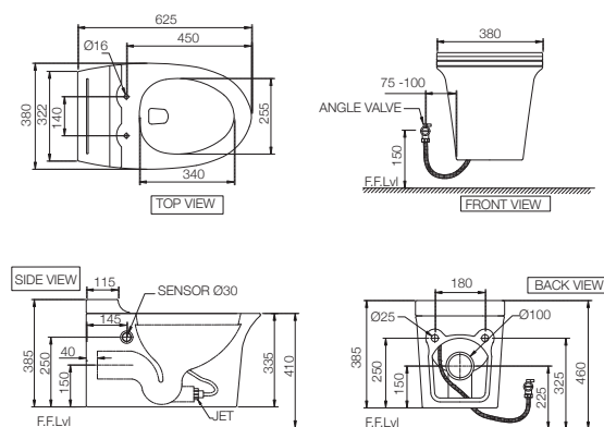
ONS-WHT-10961BIUFMSTL Tankless Wall Hung WC with Sensor Flush, UF Soft Close Slim Seat Cover, Hinges, Accessories Set, Size: 380x625x385 mm
