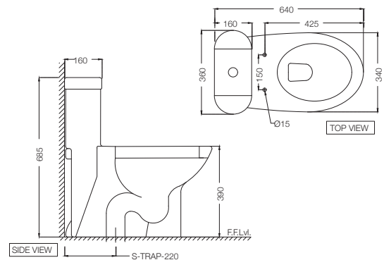
SLS-WHT-6851S220PP Single Piece WC with PP Soft Close Seat Cover, Hinges, Dual Flush Cistern Fitting, Fixing Accessories and Accessories Set, Size: 360x640x685 mm, S Trap- 220 mm
