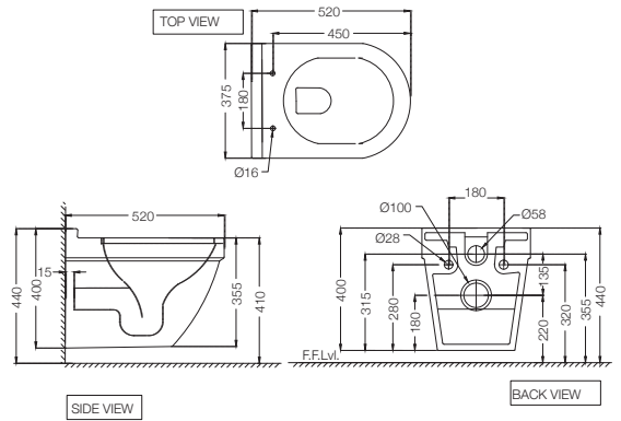
SLS-BLM-6953BIUFSM Rimless, Blind Installation Wall Hung WC In Black Matt with UF Soft Close Slim Seat Cover, Hinges and Accessories Set, Size: 375x520x400 mm
