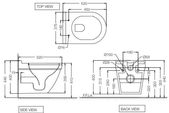
SLS-WHM-6953BIUFSM Rimless, Blind Installation Wall Hung WC In White Matt with UF Soft Close Slim Seat Cover, Hinges and Accessories Set, Size: 375x520x400 mm
