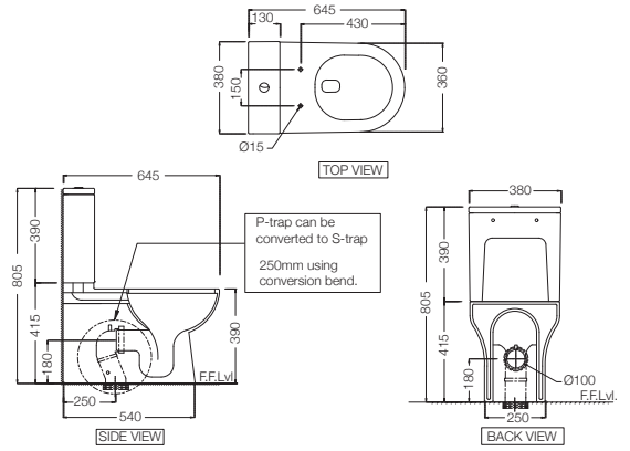
OPS-WHT-15753NS250UFSMZ Rimless Bowl with Cistern for Coupled WC with UF Soft Close Slim Seat Cover, Hinges, Dual Flush Cistern Fitting, Conversion Bend, Fixing Accessories Set, Size: 380x645x805 mm, S Trap- 250 mm (with Conversion Bend)
