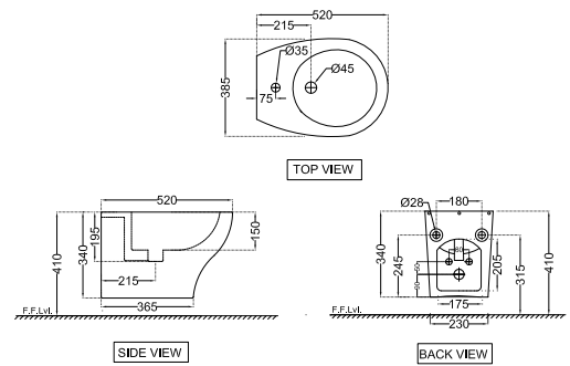
ACS-WHT-87153 Wall Hung Bidet with Accessories Set, Size: 385x520x340 mm
