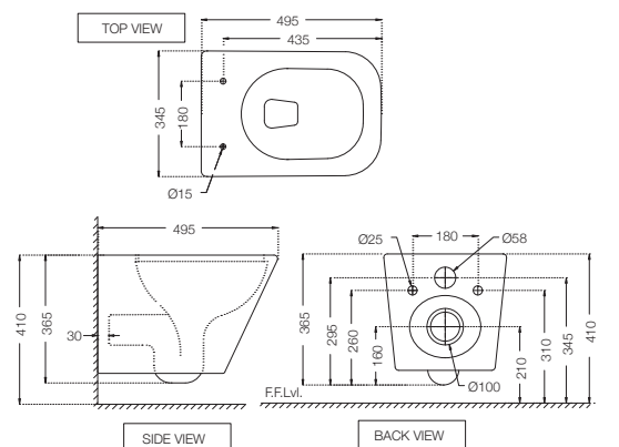
ARS-WHT-39953BIUFSM Rimless, Blind Installation Wall Hung WC with UF Soft Close Slim Seat Cover, Hinges, Accessories Set, Size: 345x495x365 mm
