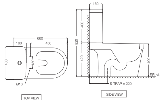
OPS-WHT-15751S220UFSMZ Bowl with Cistern for Coupled WC with UF Soft Close Slim Seat Cover, Hinges, Single Flush Cistern Fitting, Fixing Accessories and Accessories Set, Size: 400x660x820 mm, S Trap- 220 mm
