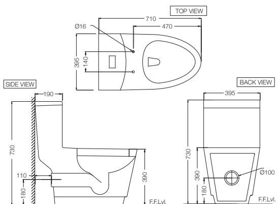
VGS-WHT-81853P180UF Rimless Single Piece WC with UF Soft Close Seat Cover, Hinges, Dual Flush Cistern Fitting, Fixing Accessories and Accessories Set, Size: 395x710x730 mm, P Trap- 180 mm
