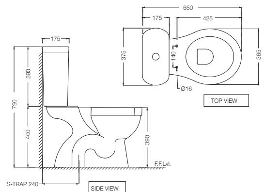
SLS-WHT-6751S240PPZ Bowl with Cistern for Coupled WC with PP Soft Close Seat Cover, Hinges, Dual Flush Cistern Fitting, Fixing Accessories and Accessories Set, Size: 375x650x790 mm, S Trap- 240 mm
