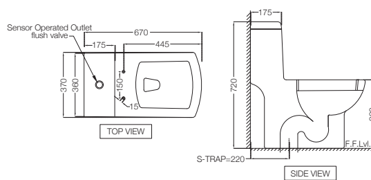
LYS-WHT-38851S220UFSMSNR Single Piece WC with UF Soft Close Slim Seat Cover, Hinges, Sensor & Manual Operated Single Flush Cistern Fitting, Fixing Accessories and Accessories Set, Size: 370x670x720 mm, S Trap- 220 mm
