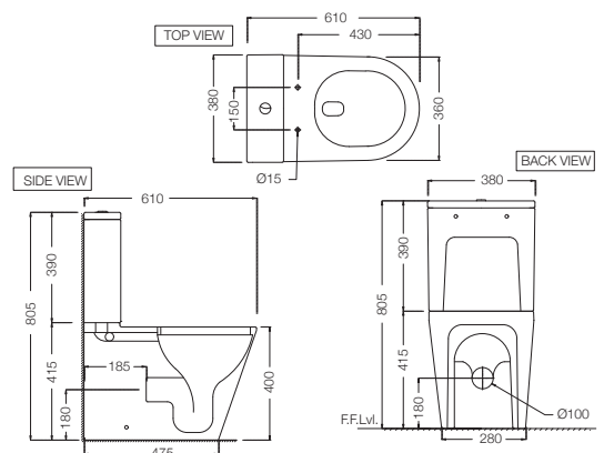
VGS-WHT-81753P180UFSMZ Rimless Bowl with Cistern for Coupled WC with UF Soft Close Slim Seat Cover, Hinges, Dual Flush Cistern Fitting, Fixing Accessories and Accessories Set, Size: 380x610x805 mm, P Trap- 180 mm
