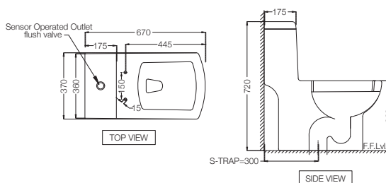
LYS-WHT-38851S300UFSMSNR Single Piece WC with UF Soft Close Slim Seat Cover, Hinges, Sensor & Manual Operated Single Flush Cistern Fitting, Fixing Accessories and Accessories Set, Size: 370x670x720 mm, S Trap- 300 mm
