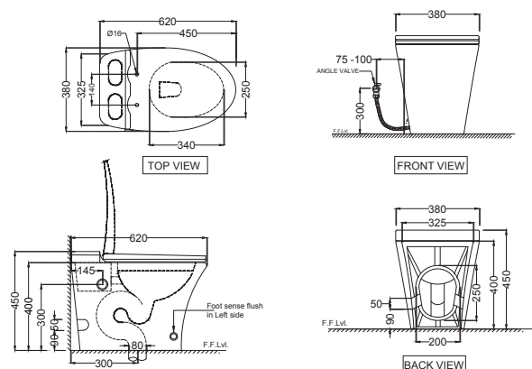
ONS-WHT-10851S300UFSMTL Tankless Single Piece WC with UF Soft Close Slim Seat Cover, Hinges, Single flush with Sensor & Manual operated, Fixing Accessories and Accessories Set, Size: 380x620x450 mm, S Trap- 300 mm
