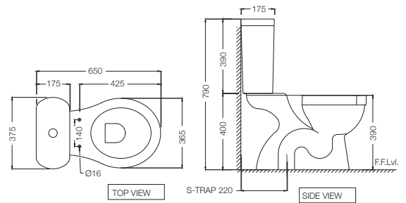
SLS-WHT-6751S220PPZ Bowl with Cistern for Coupled WC with PP Soft Close Seat Cover, Hinges, Dual Flush Cistern Fitting, Fixing Accessories and Accessories Set, Size: 375x650x790 mm, S Trap- 220 mm
