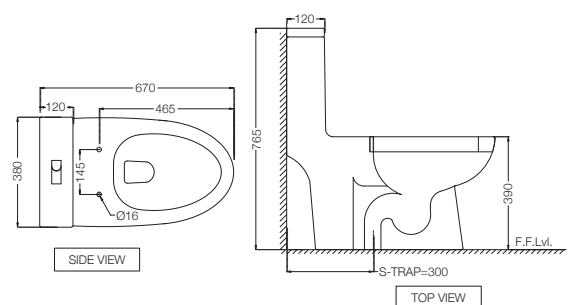
FSS-WHT-29853S300UFSM Rimless Single Piece WC with UF Soft Close Slim Seat Cover, Hinges, Dual Flush Cistern Fitting, Fixing Accessories and Accessories Set, Size: 380x670x765 mm, S Trap- 300 mm
