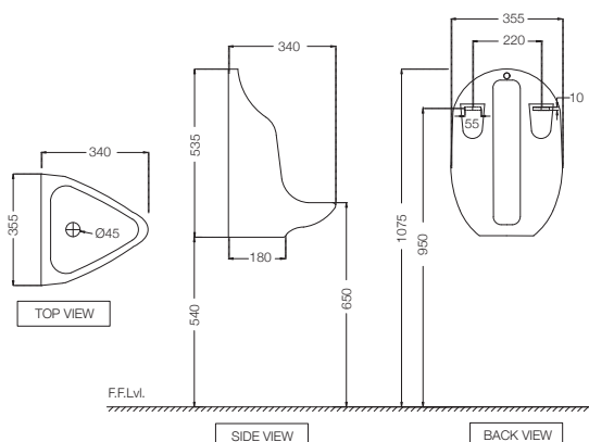
URS-WHT-13261 Urinal with Fixing Accessories, Size: 355x340x535 mm
